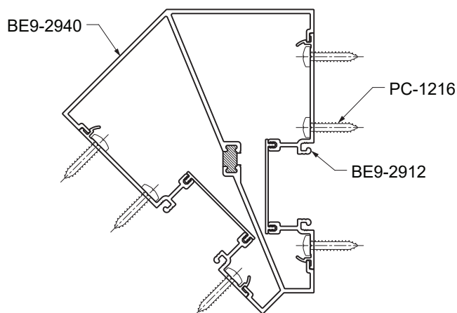
135° Inside Corner
