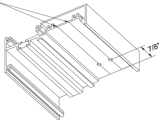
Detail 8 HORIZONTAL
