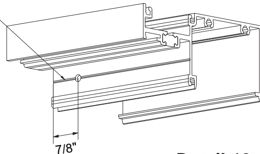
Detail 10 HORIZONTAL
