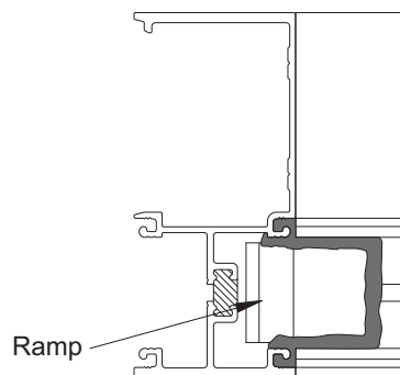
Detail 40 1" Glazing Shown
