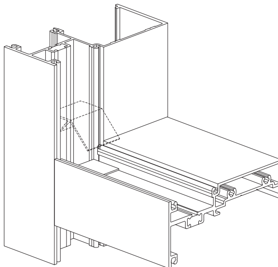
Detail 38 1" Glazing Shown
