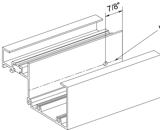
Detail 9 HEAD
