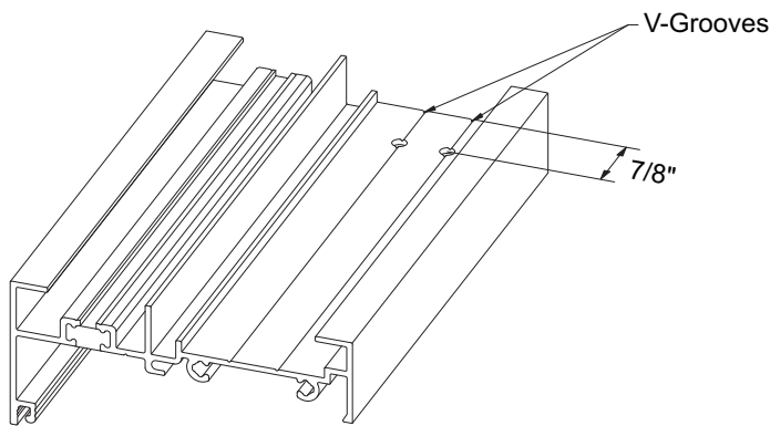
Detail 7 HEAD
