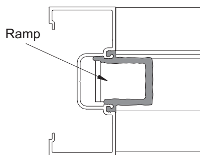
Detail 30 1" Glazing Shown 1/4" Glazing Similar
