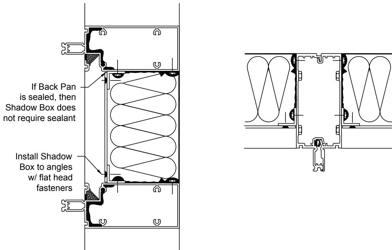
FIGURE 73 Back Pan Horizontal & Vertical Details
