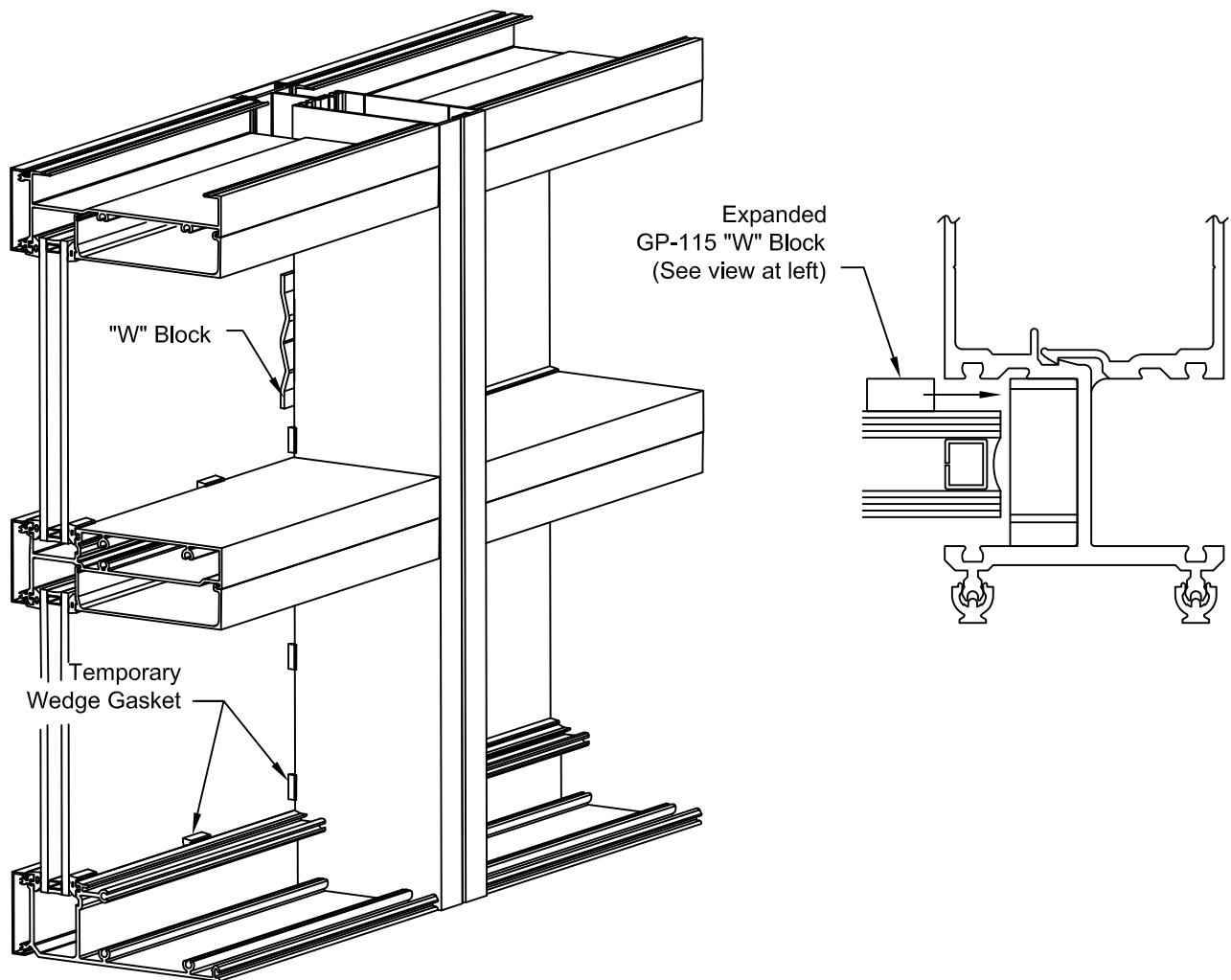
Figure 27 Glazing Retainers
