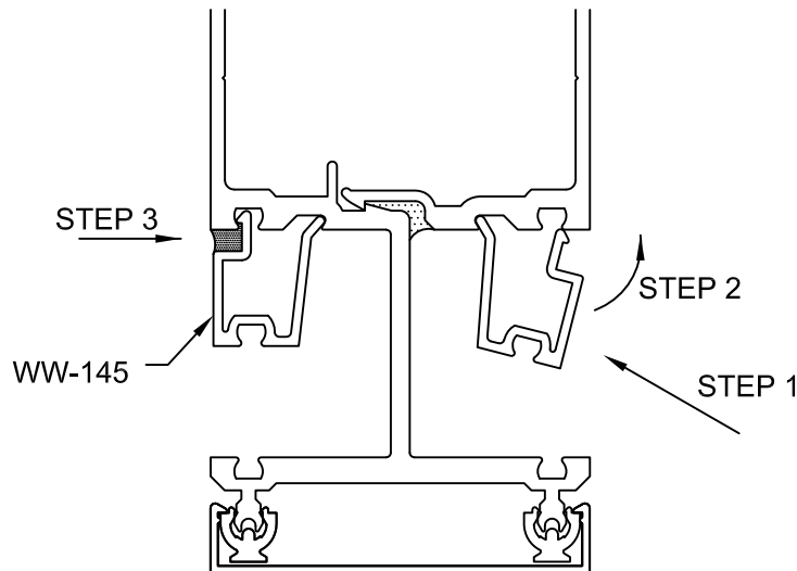
FIGURE 37 Adaptor at Typical Vertical Mullion
