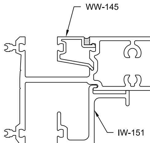
FIGURE 38 Adaptor at Typical Horizontals
