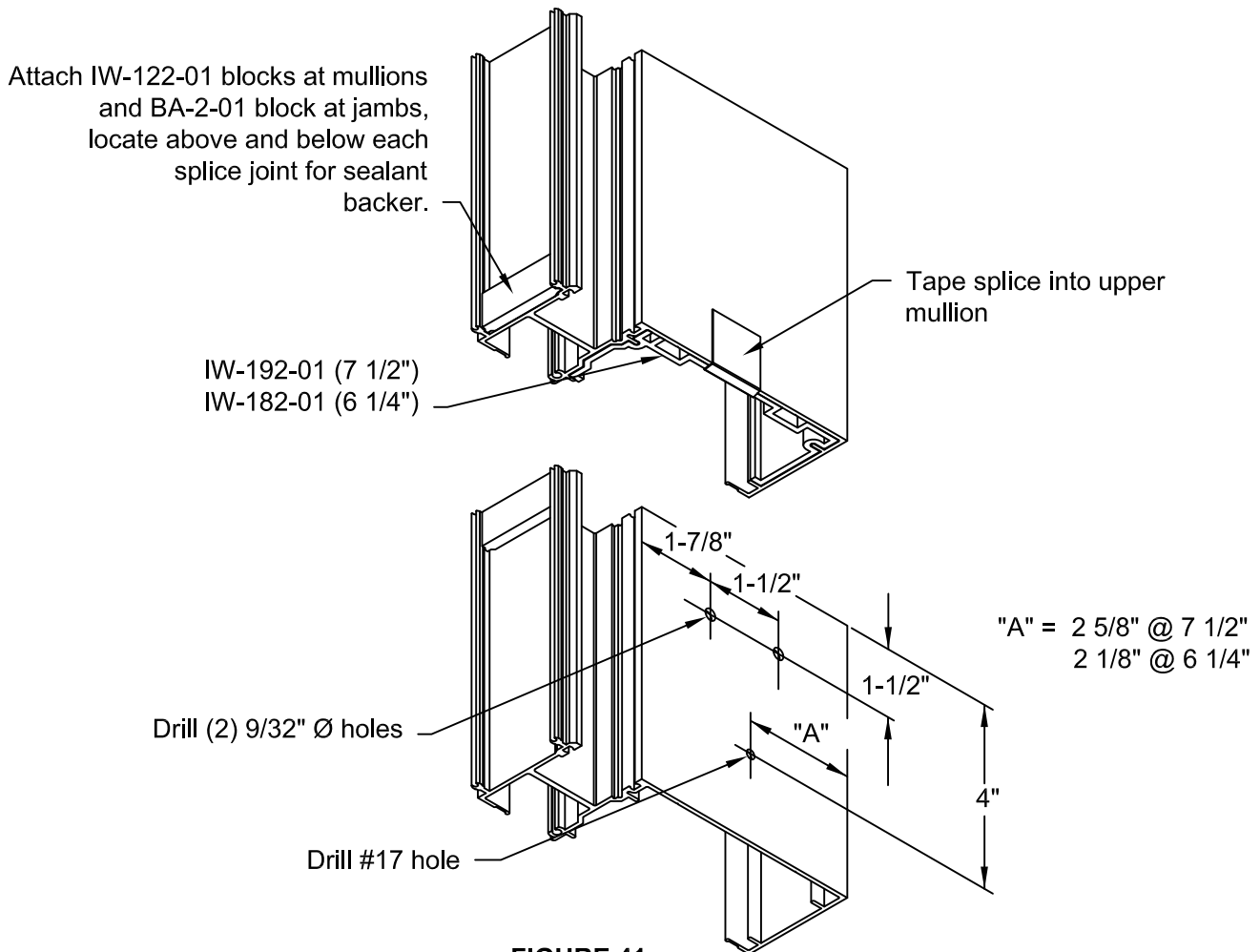
FIGURE 41 Splice Fabrication
