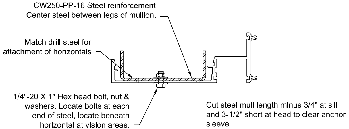
FIGURE 10 STEEL INSTALLATION
