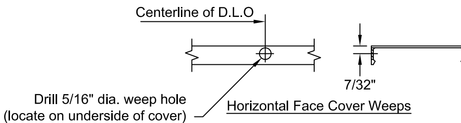
FIGURE 4 Horizontal Weep Holes
