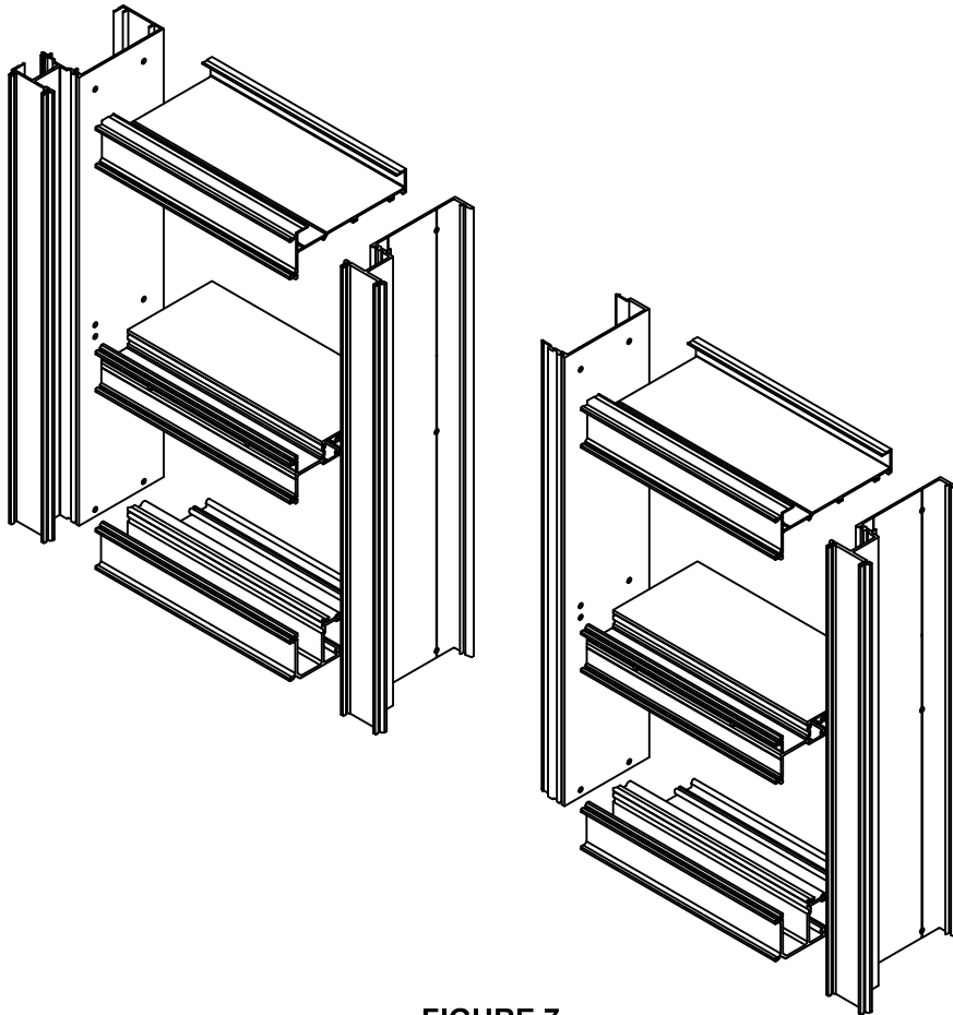
FIGURE 7 Frame Assembly
