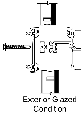
FIGURE 49 Deglazing
