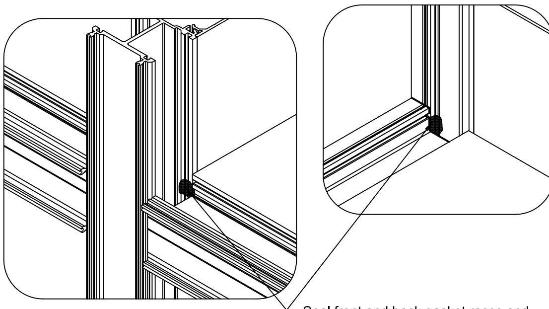
FIGURE 22 Step 1 sealant detail
