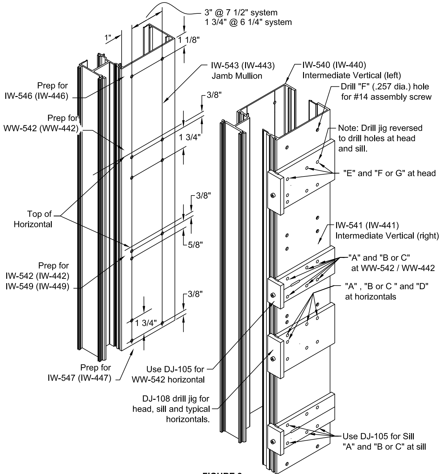
FIGURE 2 Vertical Fabrication
