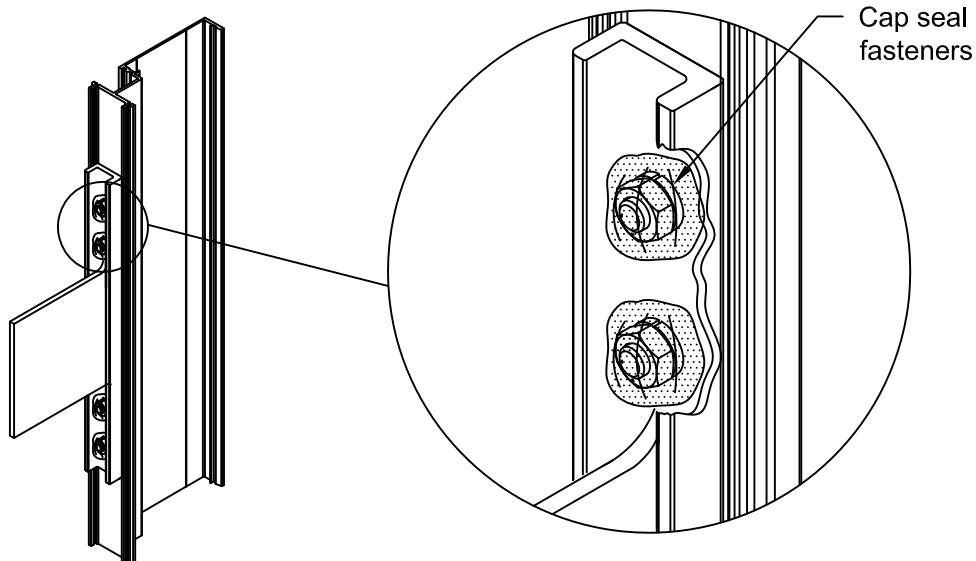
FIGURE 45 Sunshade Anchor Assembly
