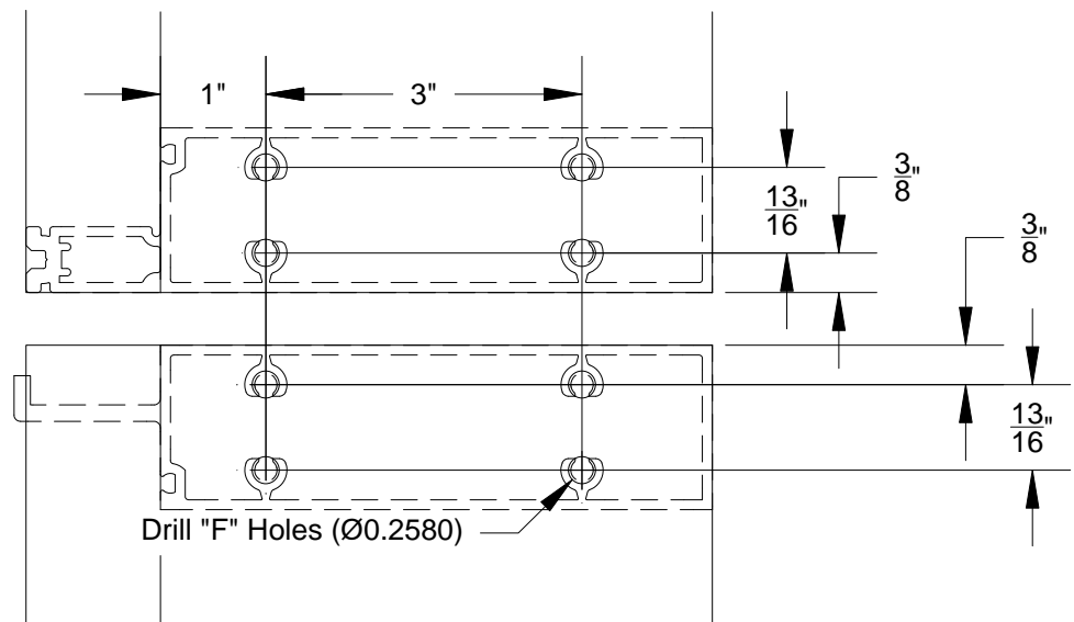
FIGURE 18 Fabrication for WW-527 & WW-528
