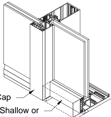
FIGURE 68 Pressure Plate & Face Caps
