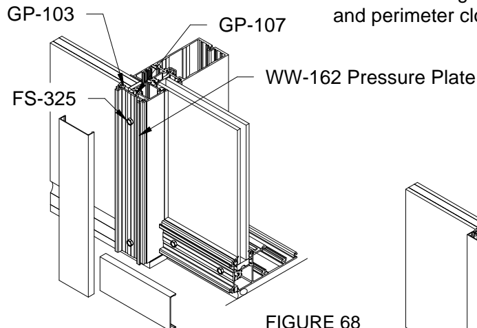
FIGURE 68 Pressure Plate & Face Caps
