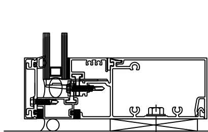
Perimeter Captured Details
