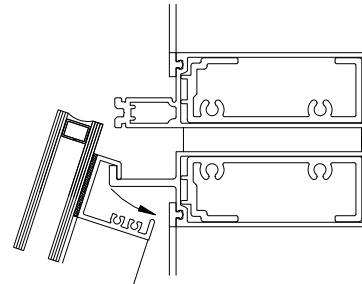
FIGURE 25 Rotate into opening and attach using cassette clips and FS-325
