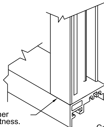
FIGURE 30 Cassette Assembly
