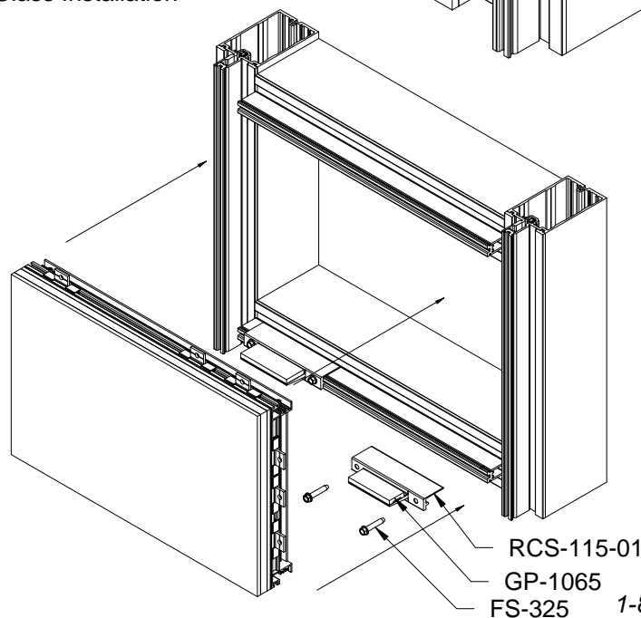
FIGURE 23 Glass Installation
