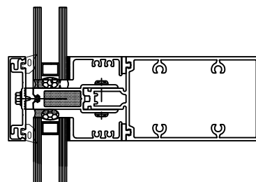
Intermediate Captured Details
