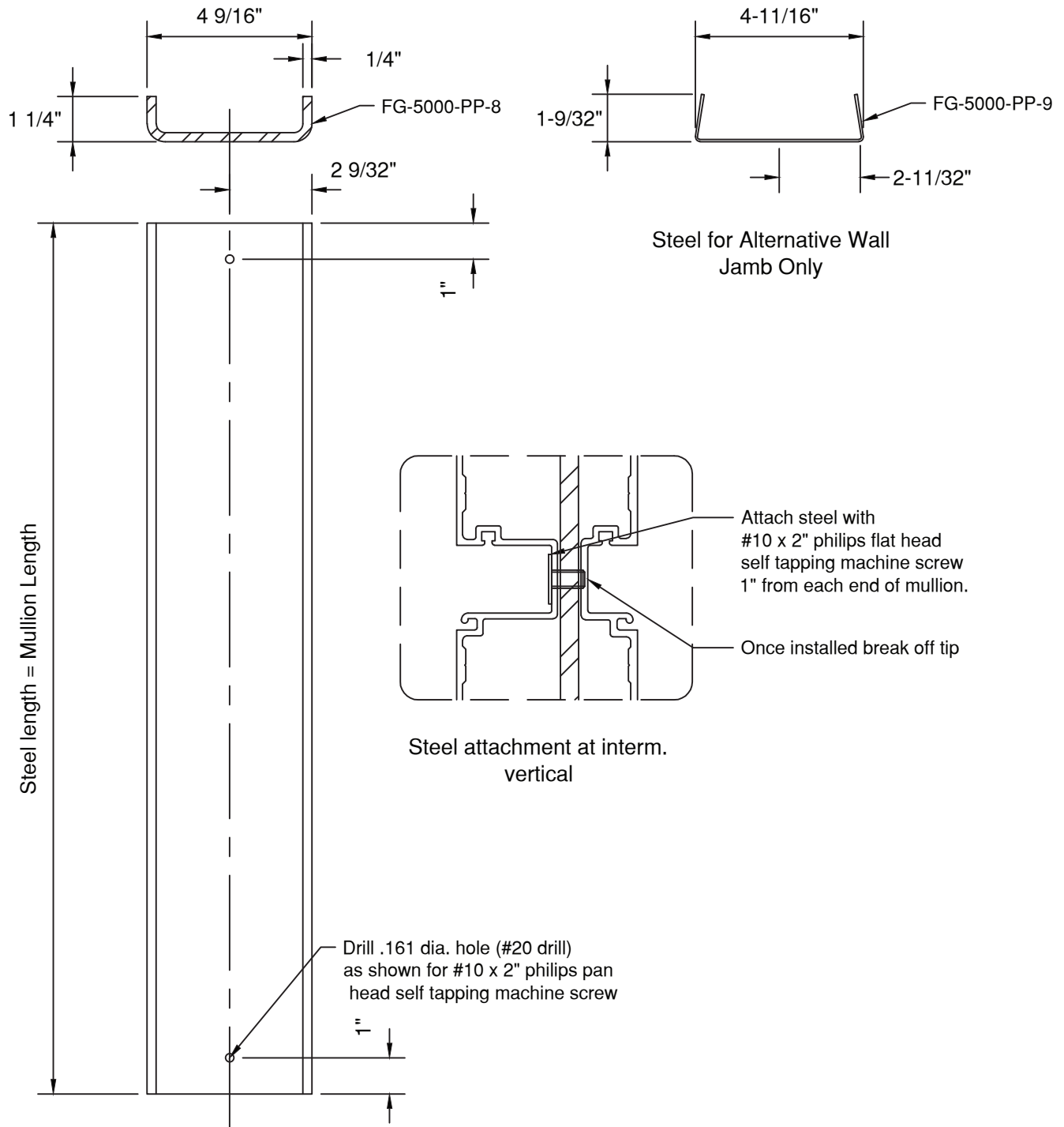
Figure 2 Steel Reinforcing
