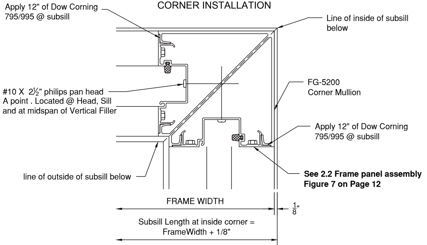
Figure 23 Inside Corner Mullion
