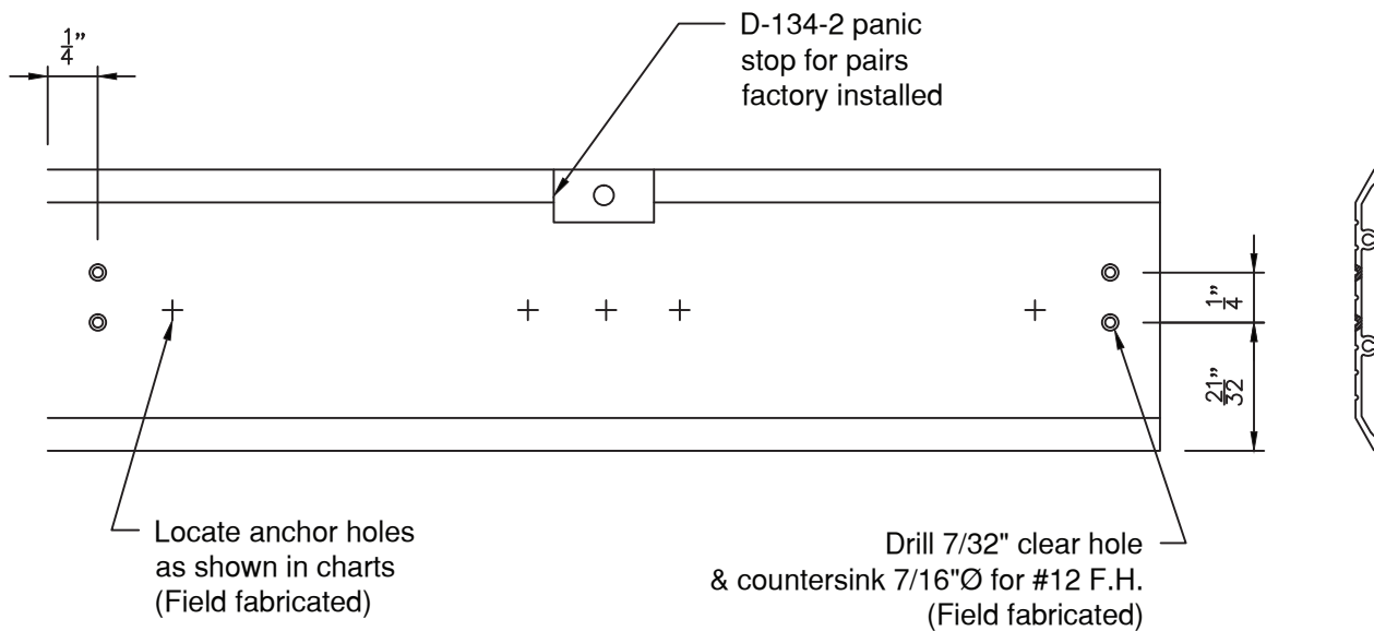
Figure 25 Threshold Fabrication
