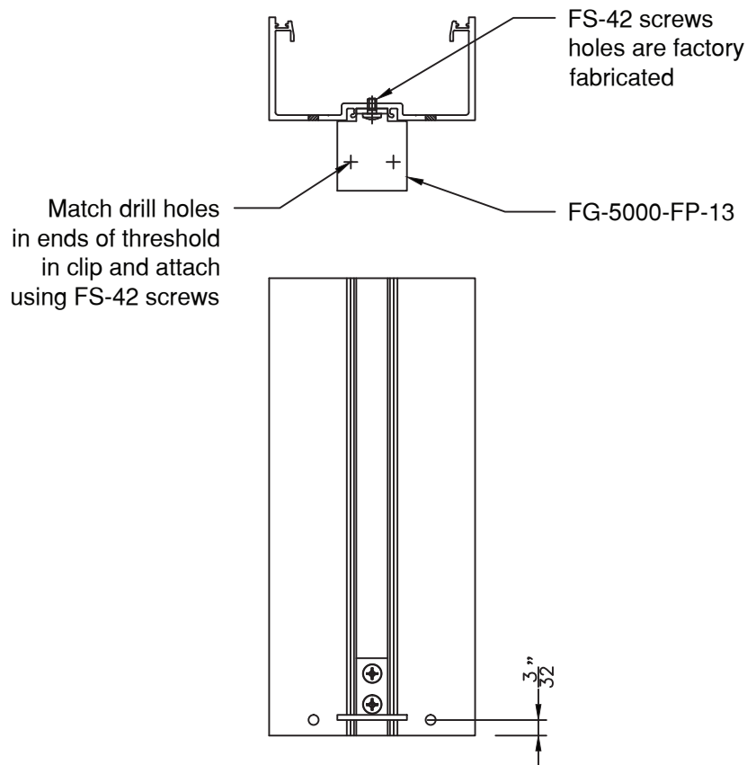
Figure 26 Alternate Threshold Attachment to Jamb
