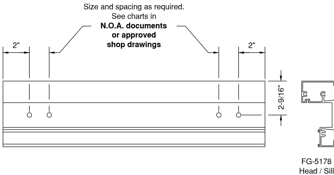
Figure 3 Head and Sill Fabrication
