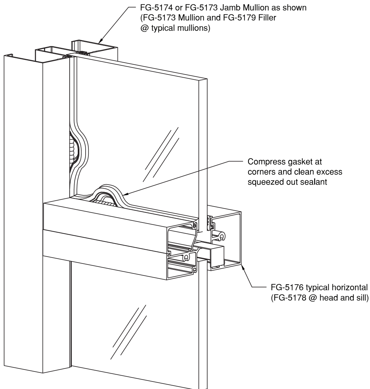
Figure 19 Compress Exterior Gasket at Corners
