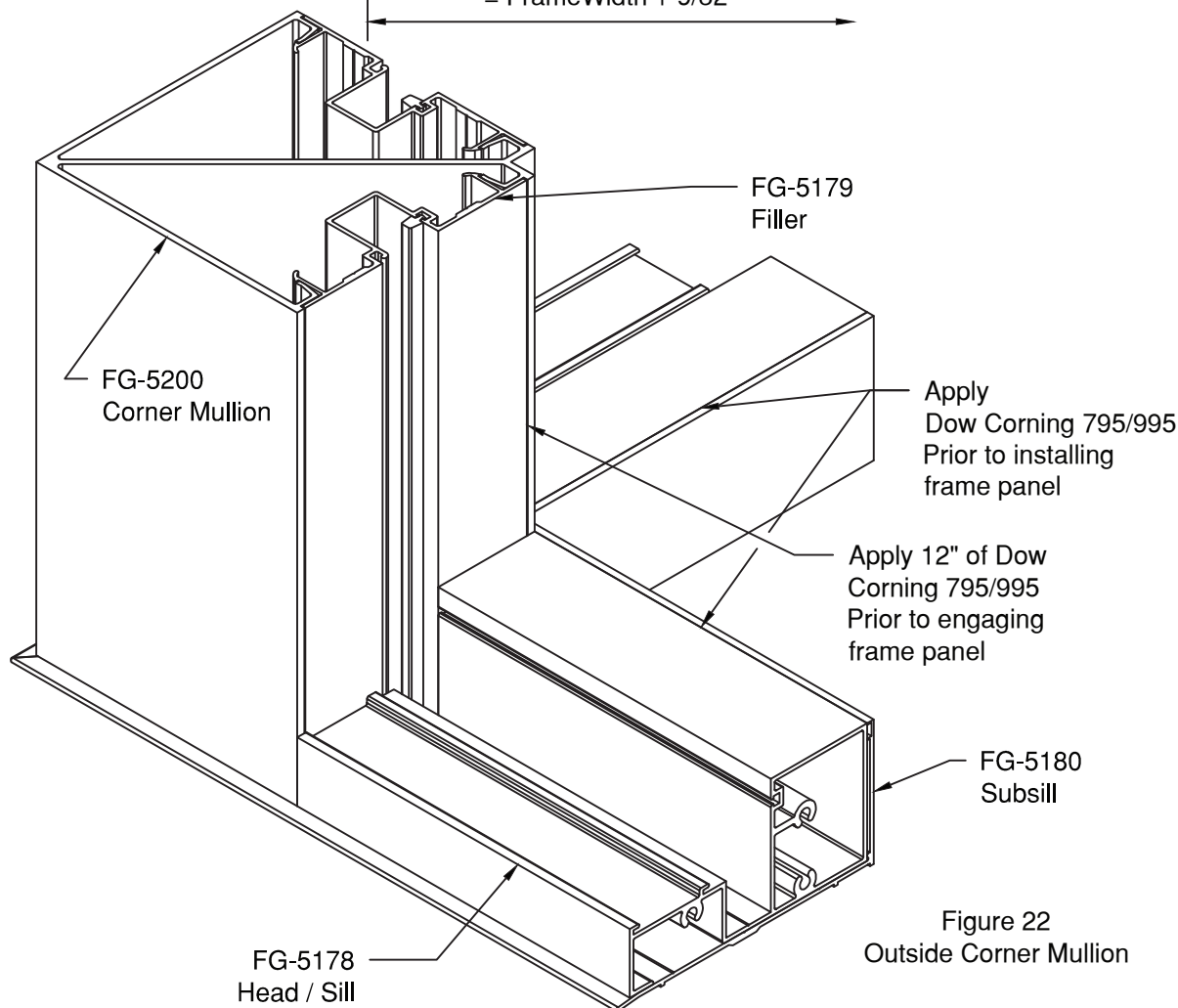
Figure 22 Outside Corner Mullion
