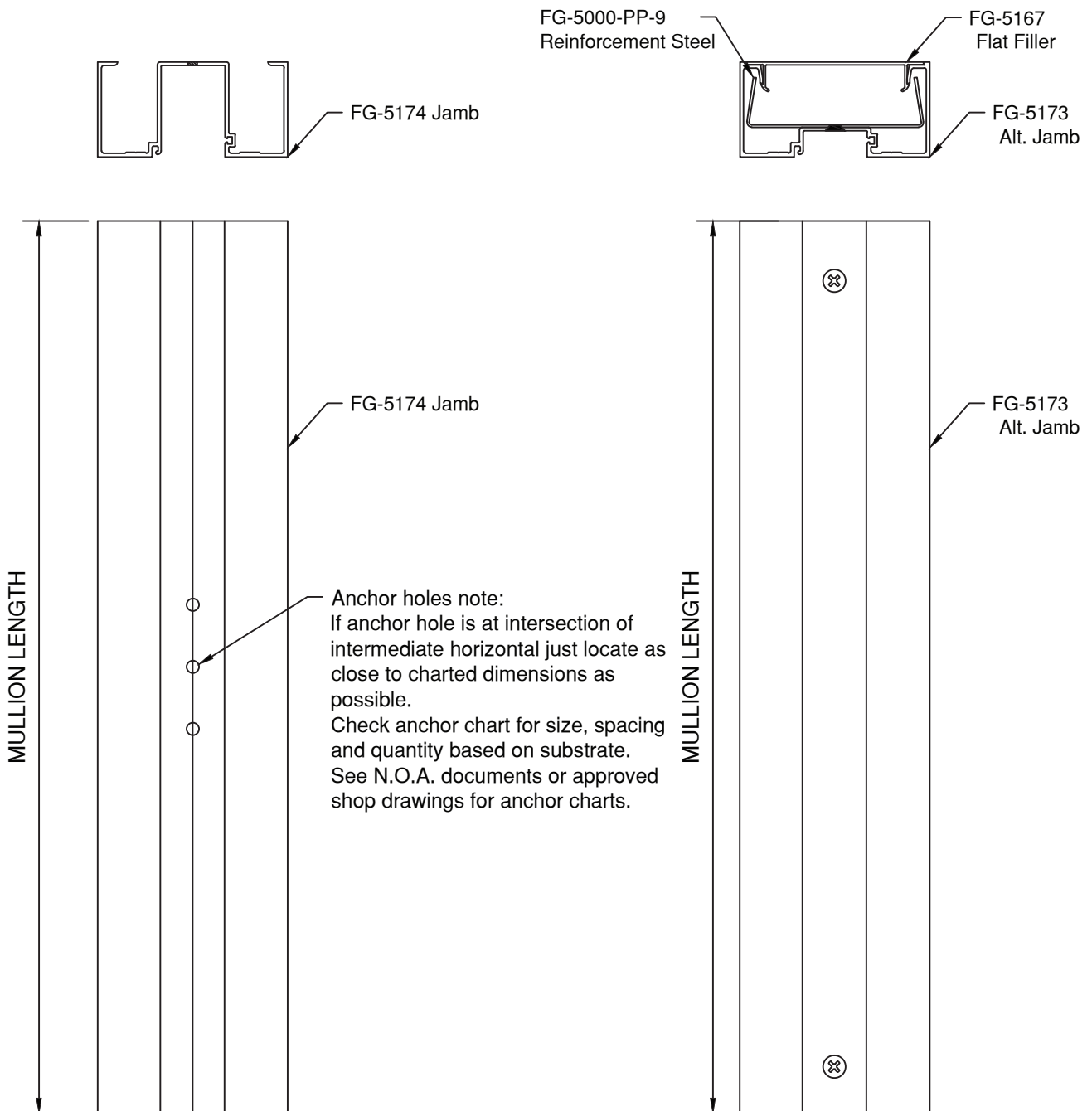
Figure 4 Jamb Fabrication
