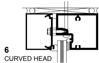
CURVED HEAD WITH ATTACHMENT CLIP
