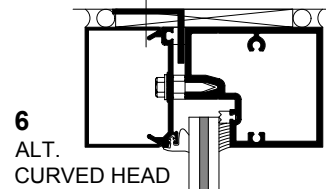
CURVED HEAD WITH ATTACHMENT CLIP
