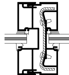
5 EXPANSION MULLION
