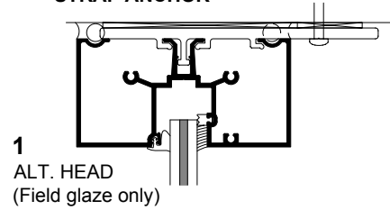
STRAP ANCHOR
