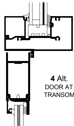
4 C.O.C. TRANSOM WITH SINGLE ACTING DOOR STOP
