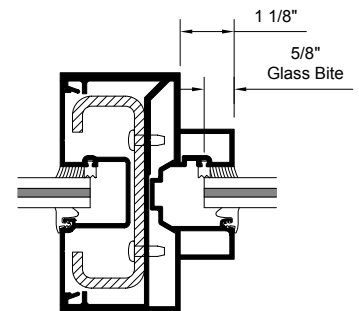
5 VERTICAL TRANSOM ABOVE DOOR
