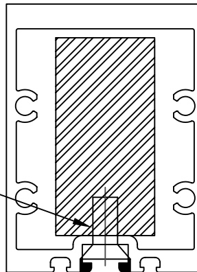
451/451T SSG TUBE MULLION WITH 1" X 2" STEEL BAR REINFORCING
