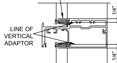
SEAL ENDS OF HORIZONTAL ADAPTORS
