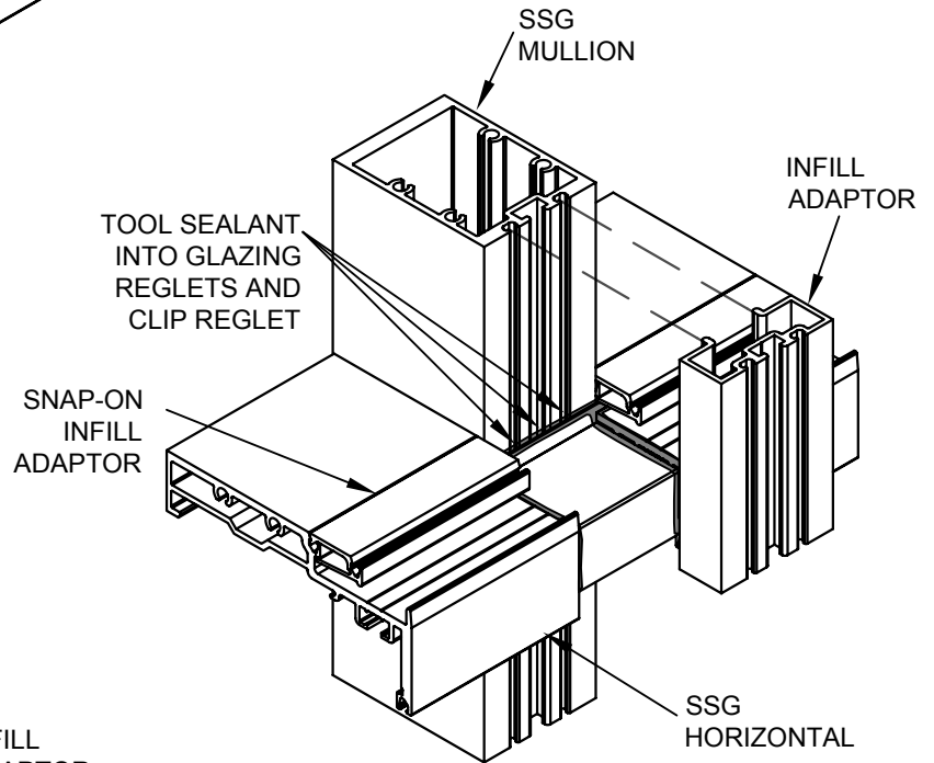
FIGURE 2 (1/4" OVER 1")
