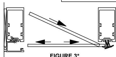
FIGURE 3* TRIFAB VG 450
