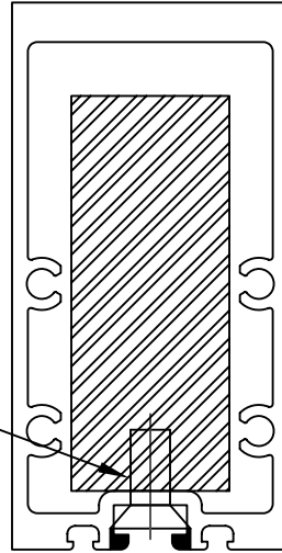
450 SSG TUBE MULLION WITH 1" X 2-1/2" STEEL BAR REINFORCING
