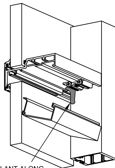
APPLY BEAD OF SEALANT ALONG VERTICAL REGLETS WHERE GLASS STOP MEETS VERTICAL
