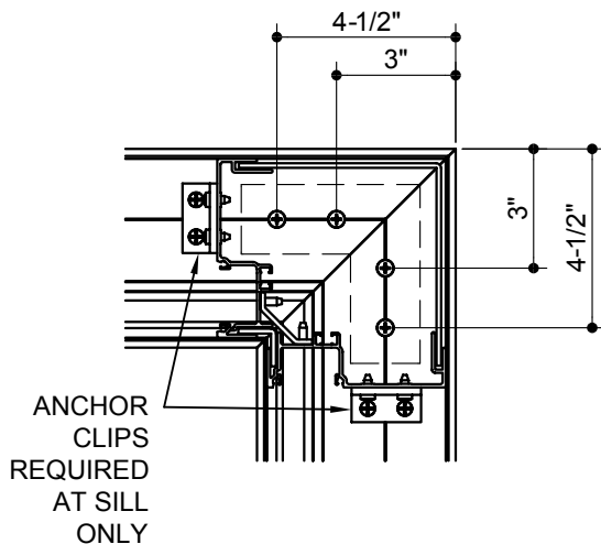
90° INSIDE CORNER
