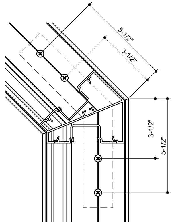
135° INSIDE CORNER
