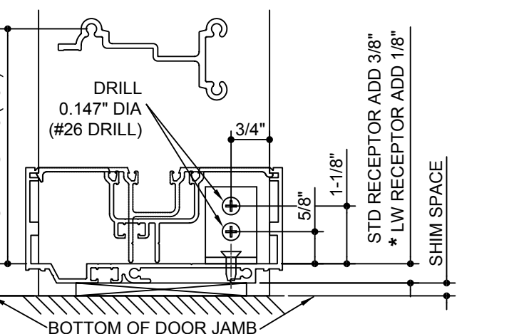
OUTSIDE OR INSIDE GLAZED - WITH OR WITHOUT TRANSOM SILL PREPS
