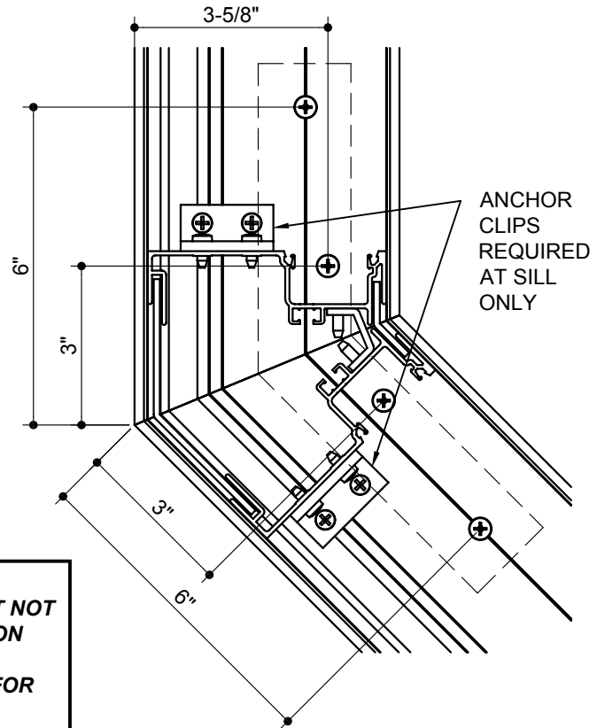
135° INSIDE CORNER
