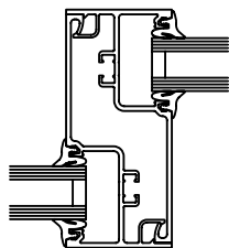
11 VERTICAL
