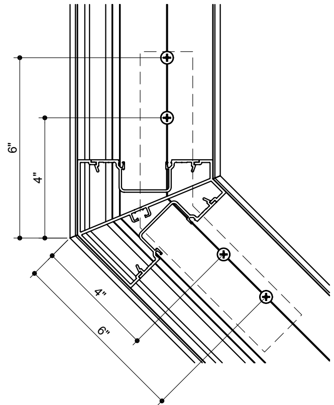
135° INSIDE CORNER
