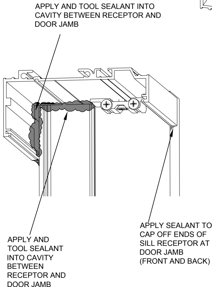
FIGURE 2 WITHOUT TRANSOM
