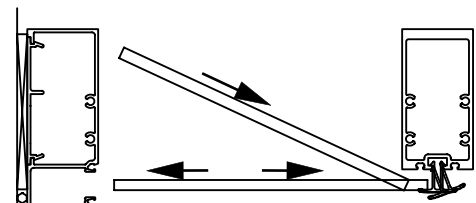
FIGURE 3* TRIFAB VG 450
