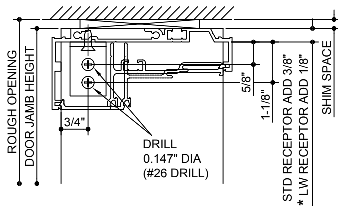
INSIDE GLAZED HEAD PREPS
