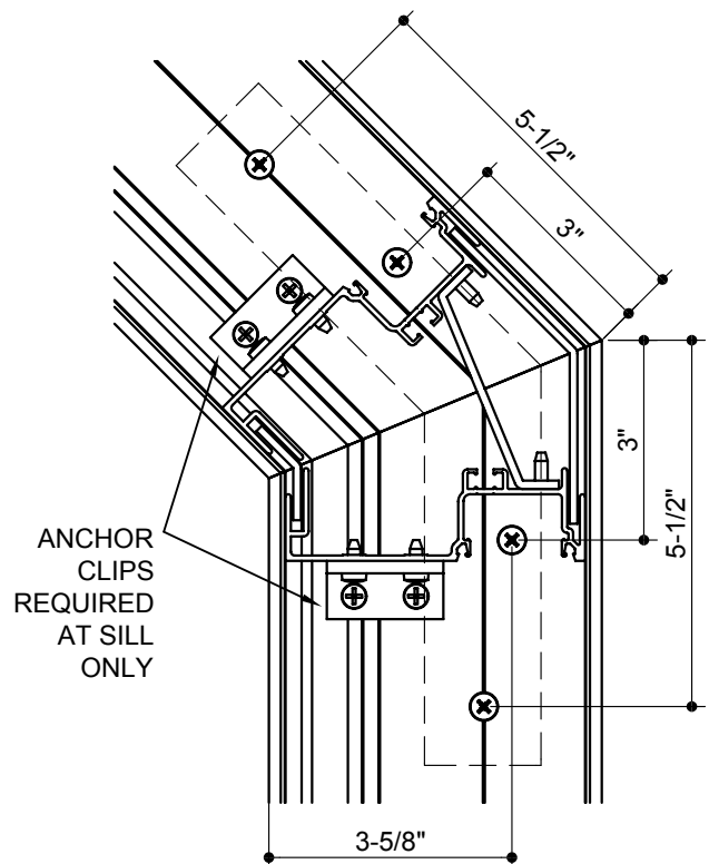
135° INSIDE CORNER
