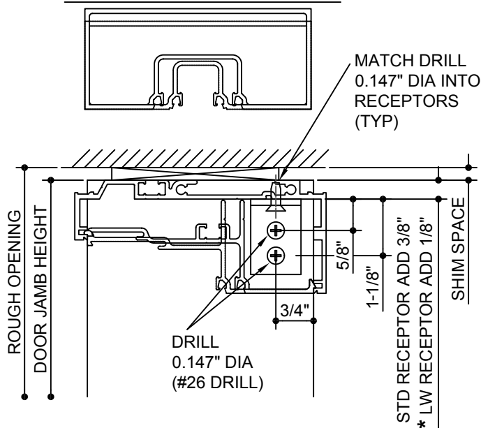
OUTSIDE GLAZED HEAD PREPS
