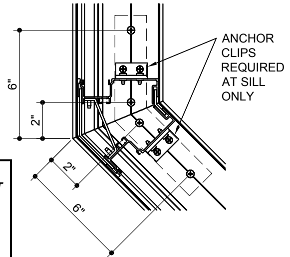
135° OUTSIDE CORNER
