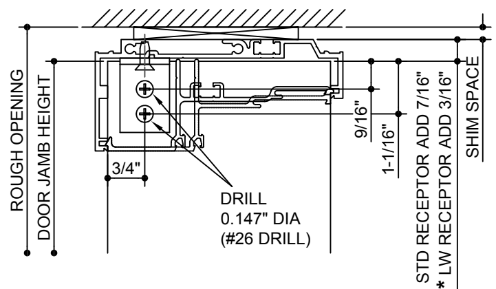
INSIDE GLAZED HEAD PREPS
