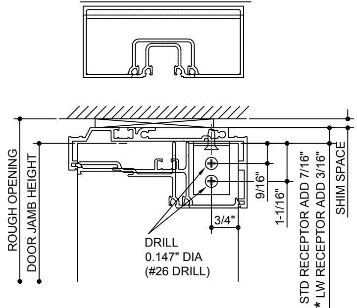
OUTSIDE GLAZED HEAD PREPS
