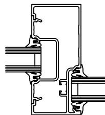
13 VERTICAL
