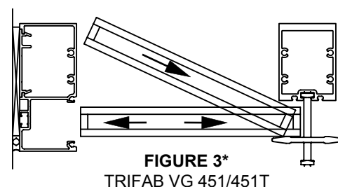
FIGURE 3* TRIFAB VG 450
