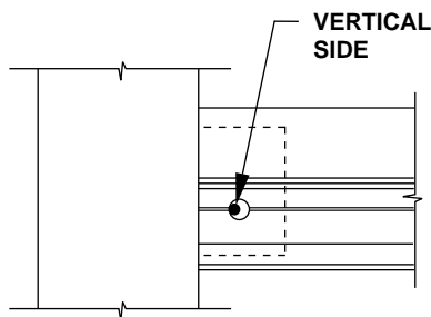
FIGURE #1 FOR CENTER OPTION INTERMEDIATE HORIZONTALS
