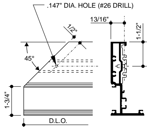
INSIDE GLAZED HORIZONTAL CUT LENGTH = D.L.O.
