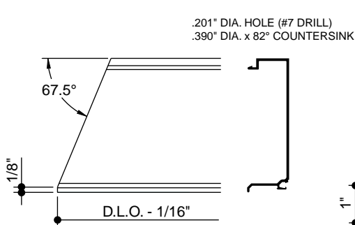
INSIDE GLAZED GLASS STOP CUT LENGTH = DLO - 1/16"
