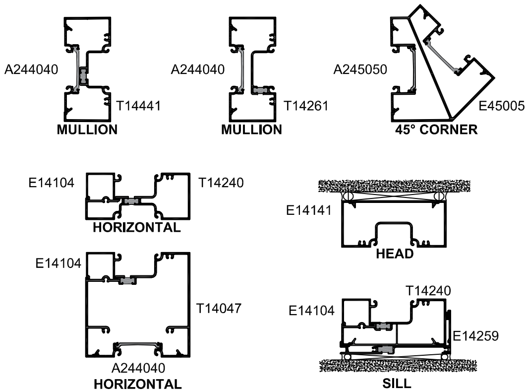
Fig 54.2 STANDARD ASSEMBLIES
