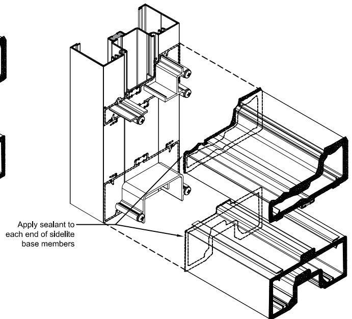
Fig.35.2 CLIP ASSEMBLY
